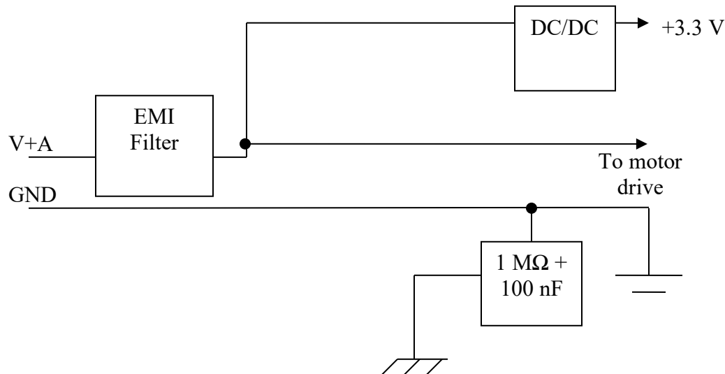
Figure 1: Power Architecture
